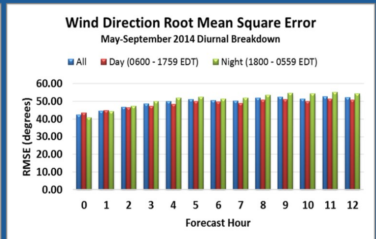
Figure 4. Same as Figure 3 but for wind direction (degrees).
