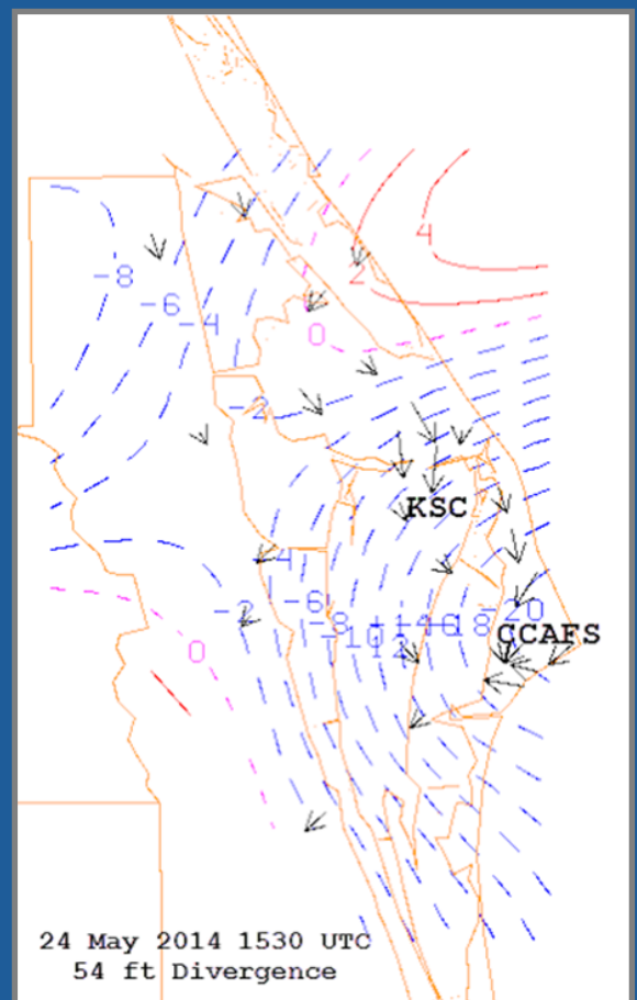
Figure 10. GEMPAK plot of wind arrows (black) from wind tower observations and divergence ( 10^{-5} \text{ sec}^{-1} ) from 24 May 2014 at 1530 UTC. Areas of convergence are shown by blue dashed lines and areas of divergence are shown by red solid lines.
