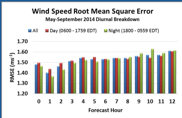
Figure 3. Wind speed ( \text{ms}^{-1} ) RMSE versus model forecast hour stratified diurnally. All values are in blue, Day values (0600-1759 EDT) are in red and Night values (1800-0559 EDT) are in green.
