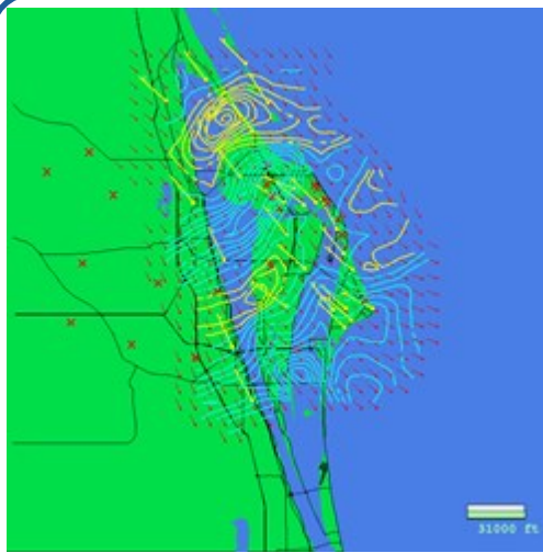
Figure 8. The MARSS system display of wind tower observations (yellow wind barbs), gridded divergence (cyan and yellow lines), and gridded wind flow vectors (red arrows). Tower locations not reporting are shown by a red x.
