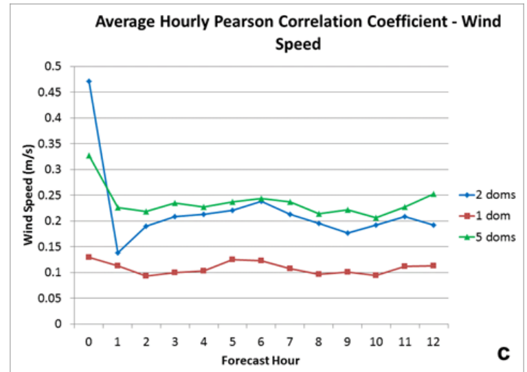
Figure 2. Charts of average hourly a) ME, b) RMSE, and c) PCC for the 12-hour wind speed forecast over the entire period of record from the three GSI/WRF configurations at the ER. In the legends, '2 doms' is the double-nest configuration (2-km outer, 0.67-km inner nest), '1 dom' is the single-domain configuration (1-km domain), and '5 doms' is the triple-nest configuration (9-km outer, 3-km middle, 1-km inner nest).
