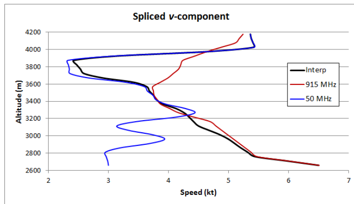
Figure 8. Example v -component (kt) profile versus altitude ( m ) for 1515 UTC 2 January 2014. Red, blue, and black lines stand for the concurrent 915-MHz, 50-MHz, and spliced DRWP profiles, respectively.
