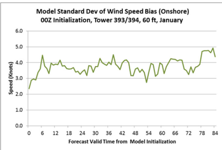
Figure 3. Onshore (left) and offshore (right) charts showing model standard deviation of bias of wind speed from a 00 UTC model initialization at SLC 39A using observations from sensors at Towers 0393 and 0394 at a sensor height of 60 ft for January 2007-2011.
