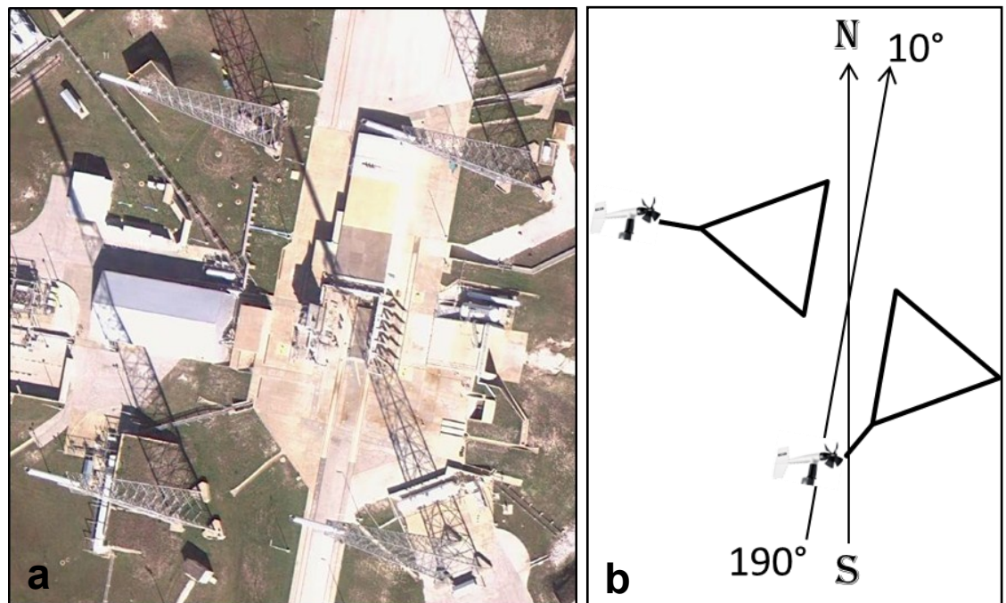
Figure 3. a) Google Earth image of the lightning protection towers at SLC 41 and b) tower shape and orientation, and sensor location. The drawing in 3b is not to scale.
