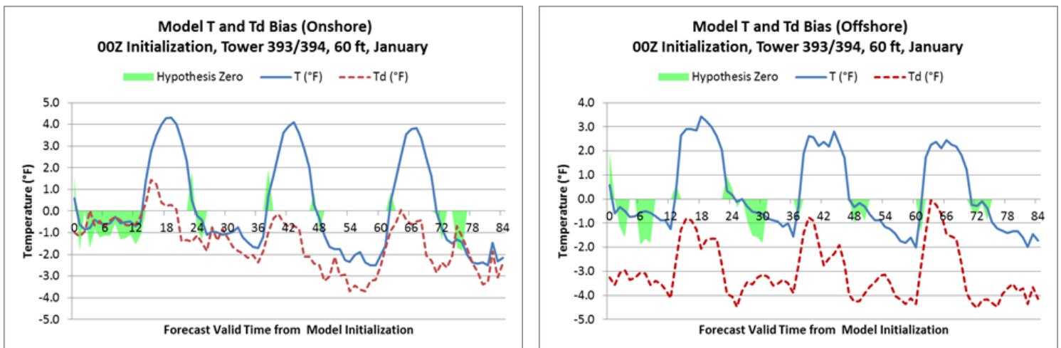
Figure 1. Onshore (left) and offshore (right) charts showing model bias of T (blue line) and Td (red dashed line) and the hypothesis zero results (green) from a 00 UTC model initialization at SLC 39A using observations from sensors at Towers 0393 and 0394 at a height of 60 ft for January 2007-2011.
