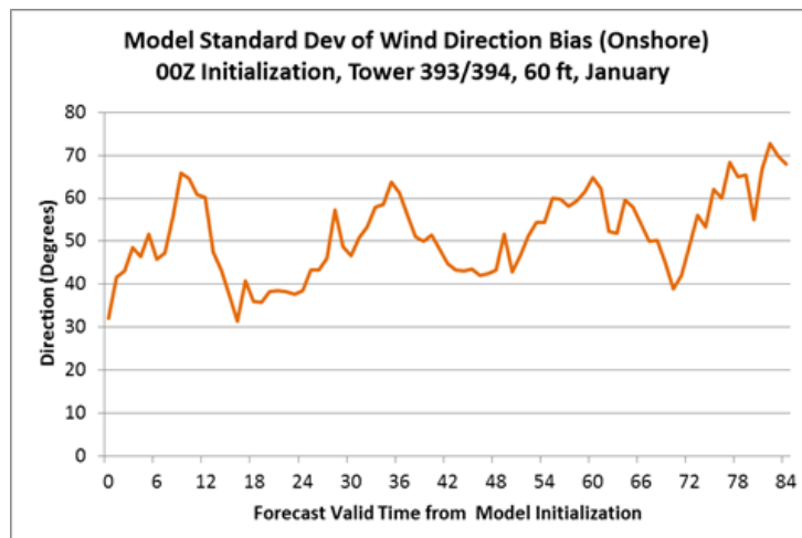
Figure 4. As in Figure 3 except for wind direction.
