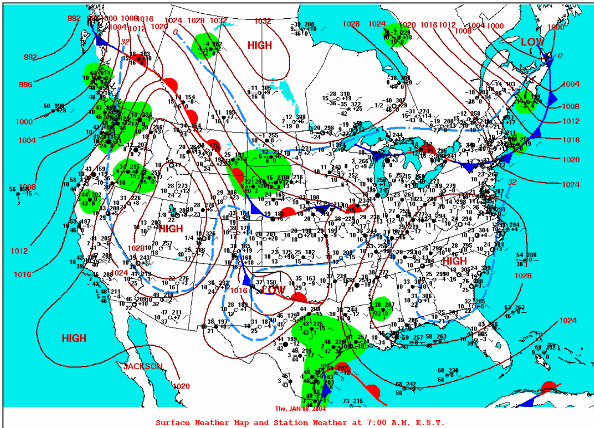
Figure 1. Surface analysis at 1200 UTC 8 January 2004.
