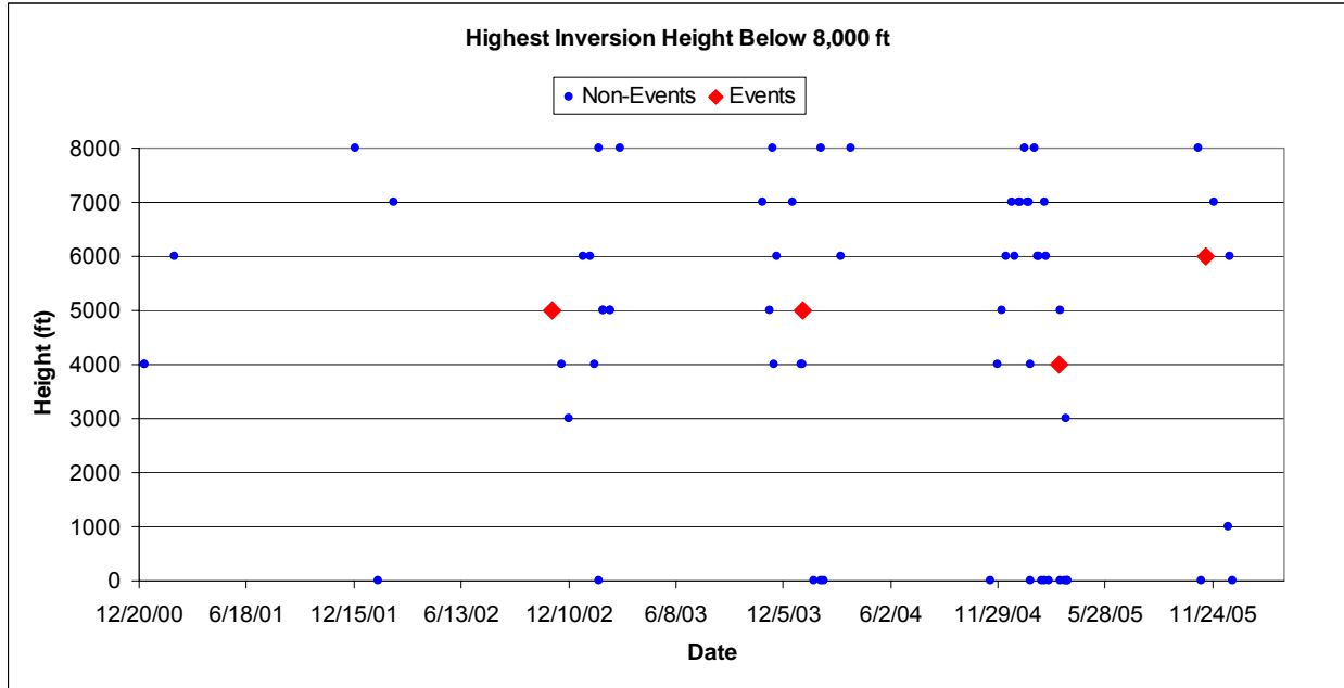
Figure 9. Scatter plot of the base of the highest inversions below 8000 ft (in ft) during events (large red diamond) and non-events (small blue circle).
