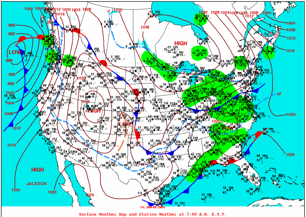
Figure 2. Surface analysis at 1200 UTC 9 January 2004.
