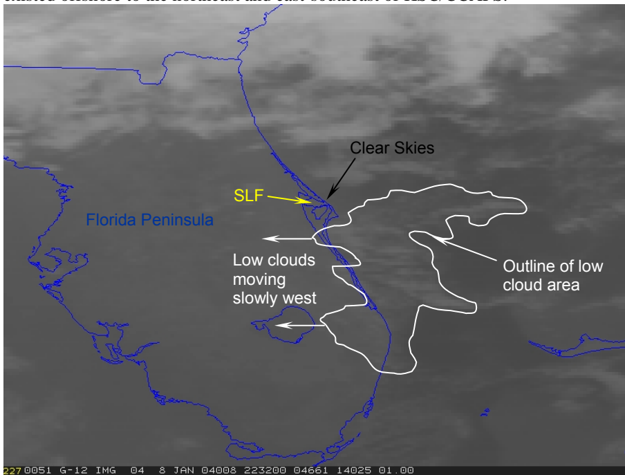
Figure 6. Infrared satellite imagery from 8 January 2004 at 2232 UTC. Clouds were still evident over the ocean northeast and east-southeast of KSC/CCAFS and skies were clear at the SLF.
