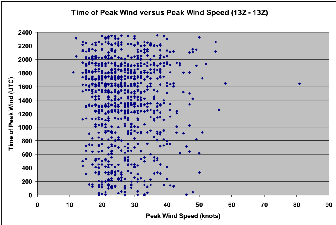
Figure 33. Scatter diagram showing the speed (knots) and time (UTC) of each observed PWS in the task, for the 24-hour period.
