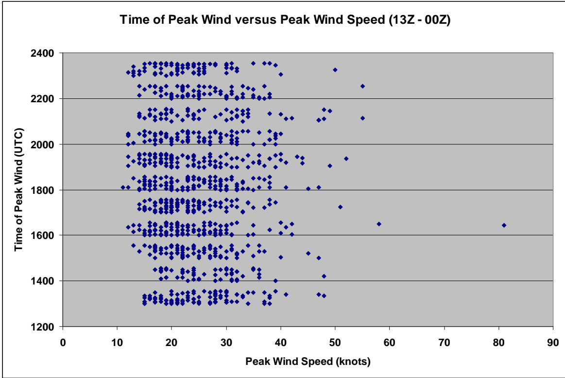
Figure 32. Scatter diagram showing the speed (knots) and time (UTC) of each observed PWS in the task, for the 11-hour period.
