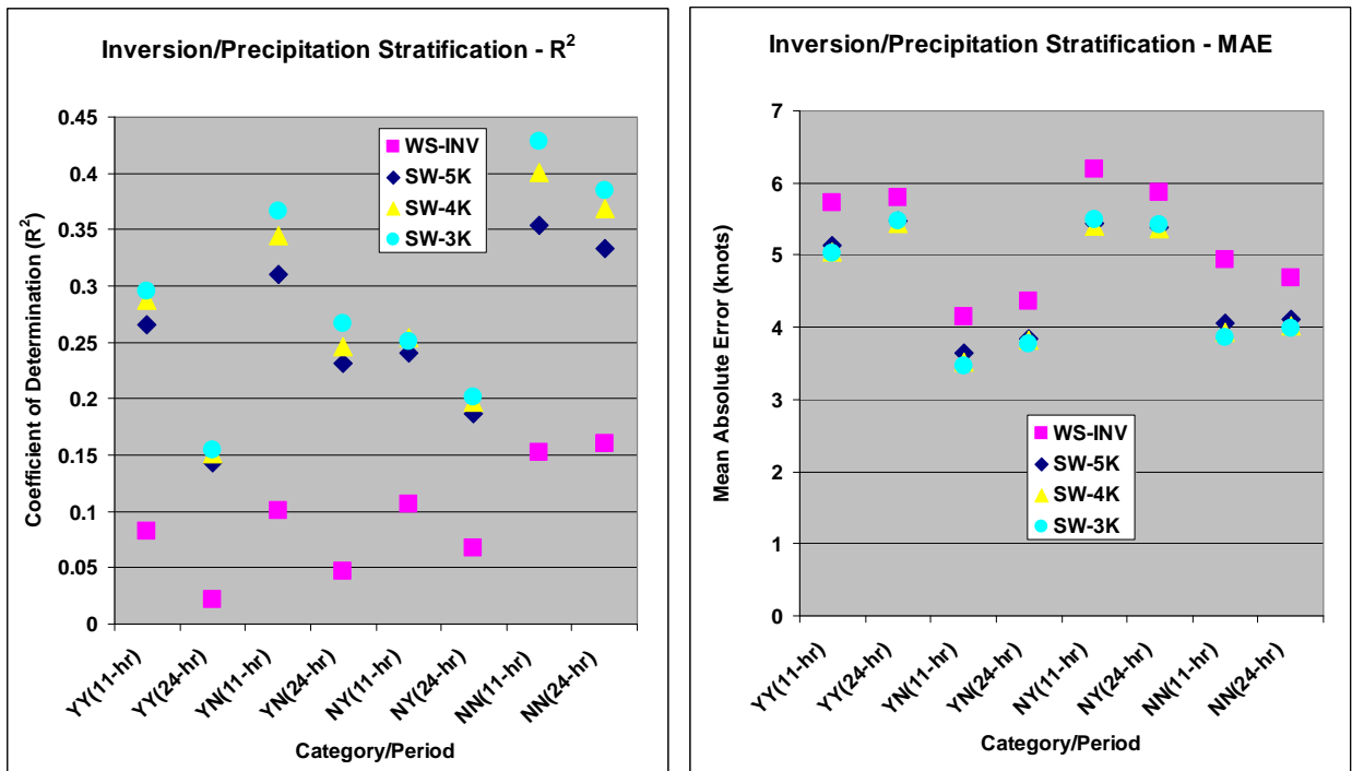
Figure 19. R^2 and MAE values for several predictors for the 11-hour and 24-hour periods, using the inversion/precipitation stratification.
