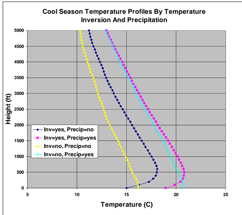
Figure 14. Average vertical profiles of temperature (C) for the four inversion (Inv)/precipitation (Precip) stratification categories. The legend shows the colors and symbols used for each profile.
