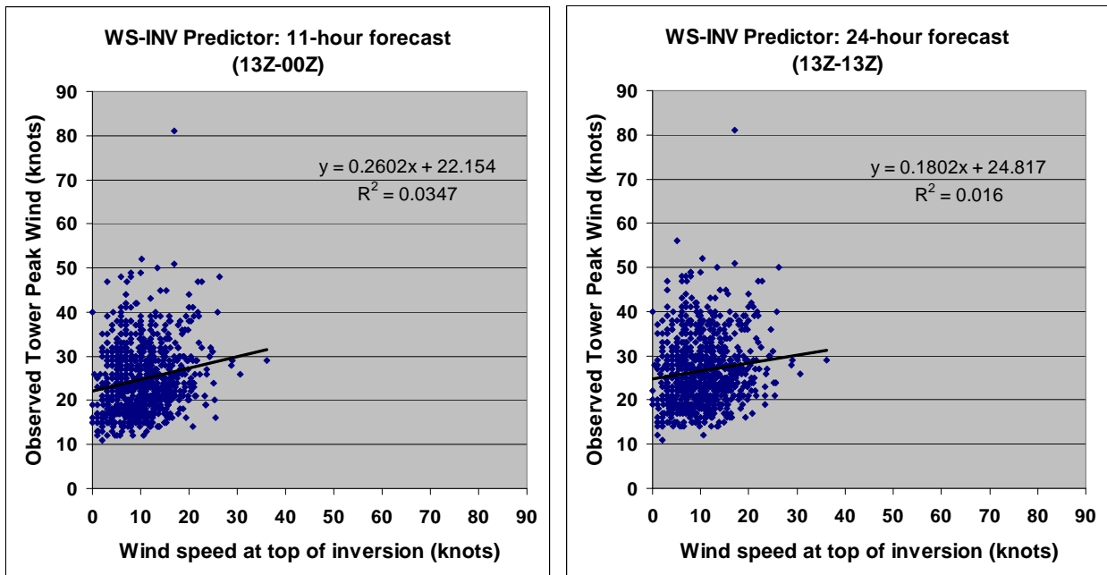
Figure 8. Scatter plots of observed PWSD versus the wind speed at the top of the inversion in the sounding for the 11-hour and 24-hour periods. The linear regression line, regression equation, and R^2 value are overlaid on the data points.
