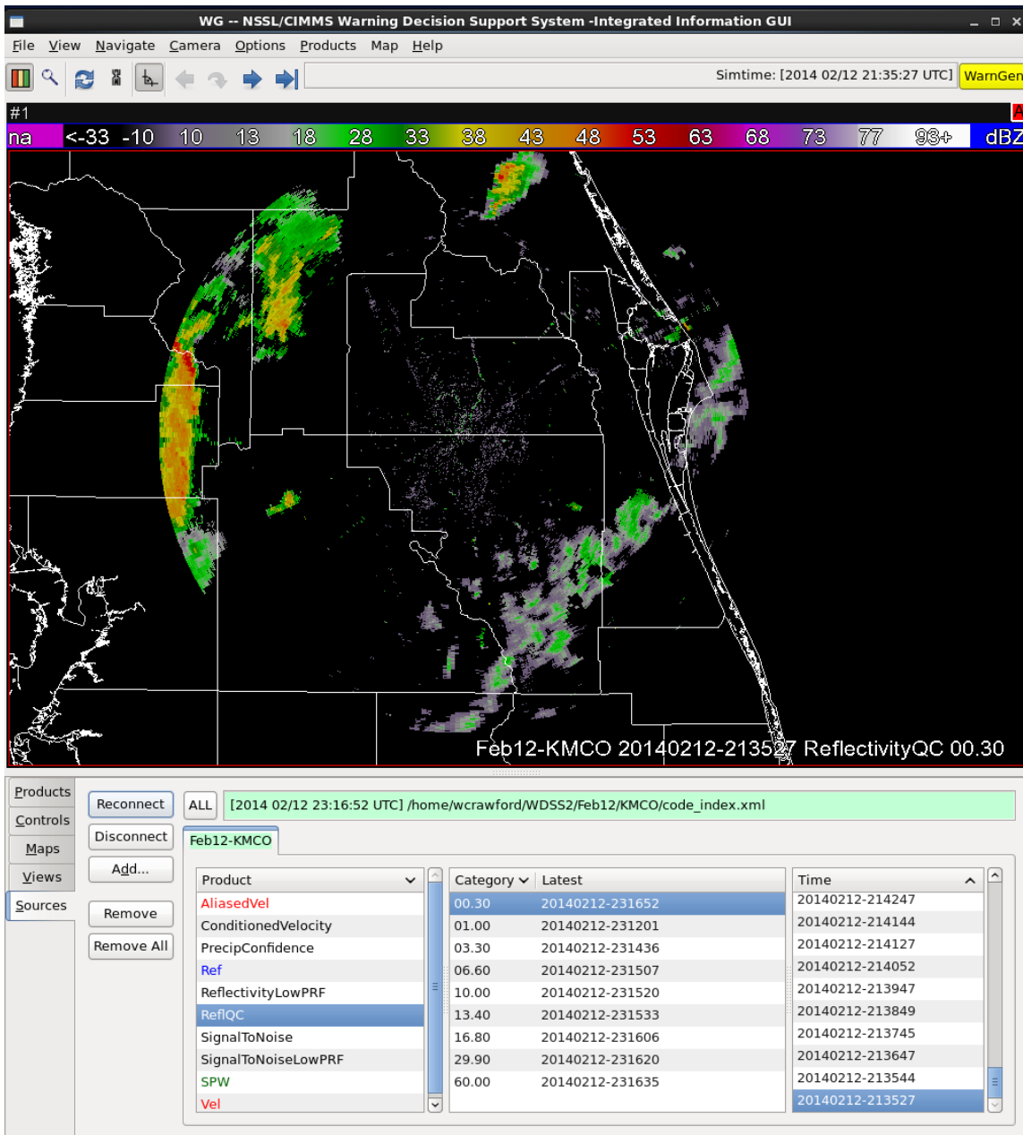
Figure 6. The WDSII GUI with data and map background displayed. The Sources section contains a tab named “Feb12-KMCO” with the choices of radar product (left column), elevation angle (middle column), and scan time (right column) for KMCO on 12 February 2014. The highlighted items in each list determine what is displayed: the 0.3° QC’d reflectivity at 213527 UTC.
