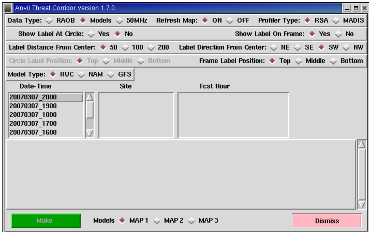
Figure 21. Anvil Tool GUI after the user has selected Anvil Tool... from the AWIPS Tools dropdown menu and selected Models as the Data Type.
