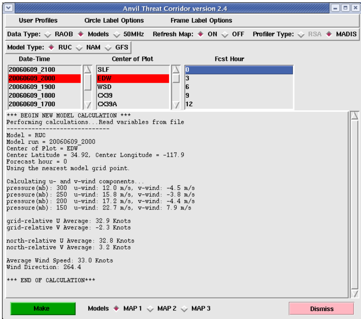
Figure 23. Anvil Tool GUI after the user has selected the model initialization time (Date-Time), location (Center of Plot), and forecast hour (Fcst Hour).
