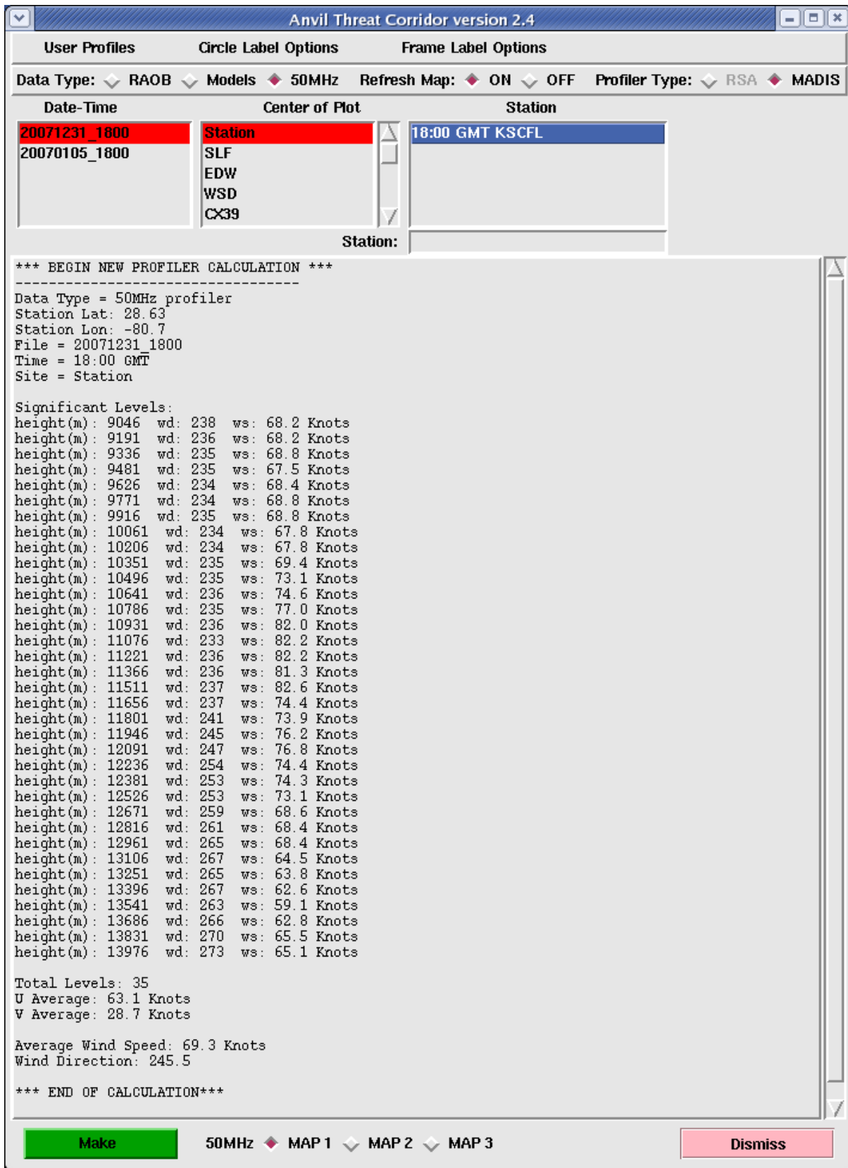
Figure 17. Anvil Tool GUI after the user selected 18:00 GMT as the profiler time in the Station listbox.
