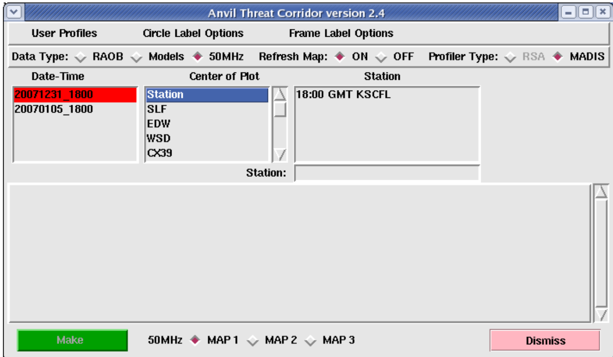
Figure 16. Anvil Tool GUI after a user has selected a Date-Time of 20071231_1800 (31 December 2007, 1800 UTC), which is highlighted in red. All of the observation times in the file are displayed in the Station listbox.
