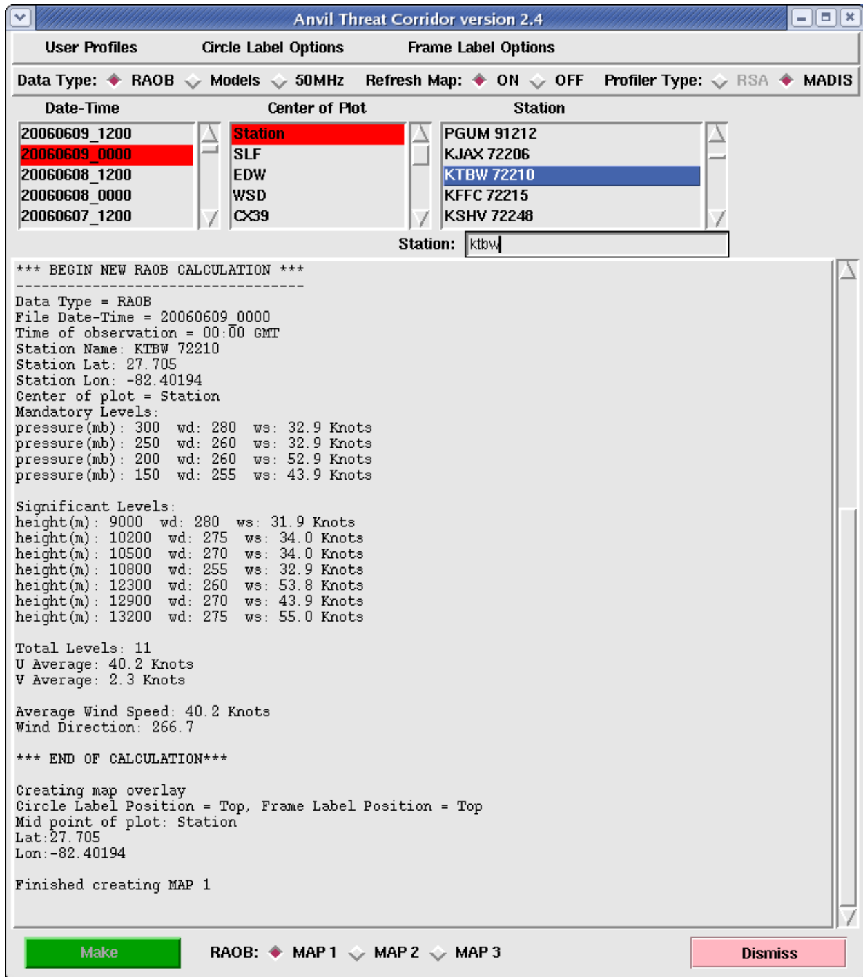
Figure 13. Anvil Tool GUI after the user has clicked on the Make button. The name and latitude/longitude of the Center of Plot, as well as the label positions, are displayed at the bottom of the GUI's text box.
