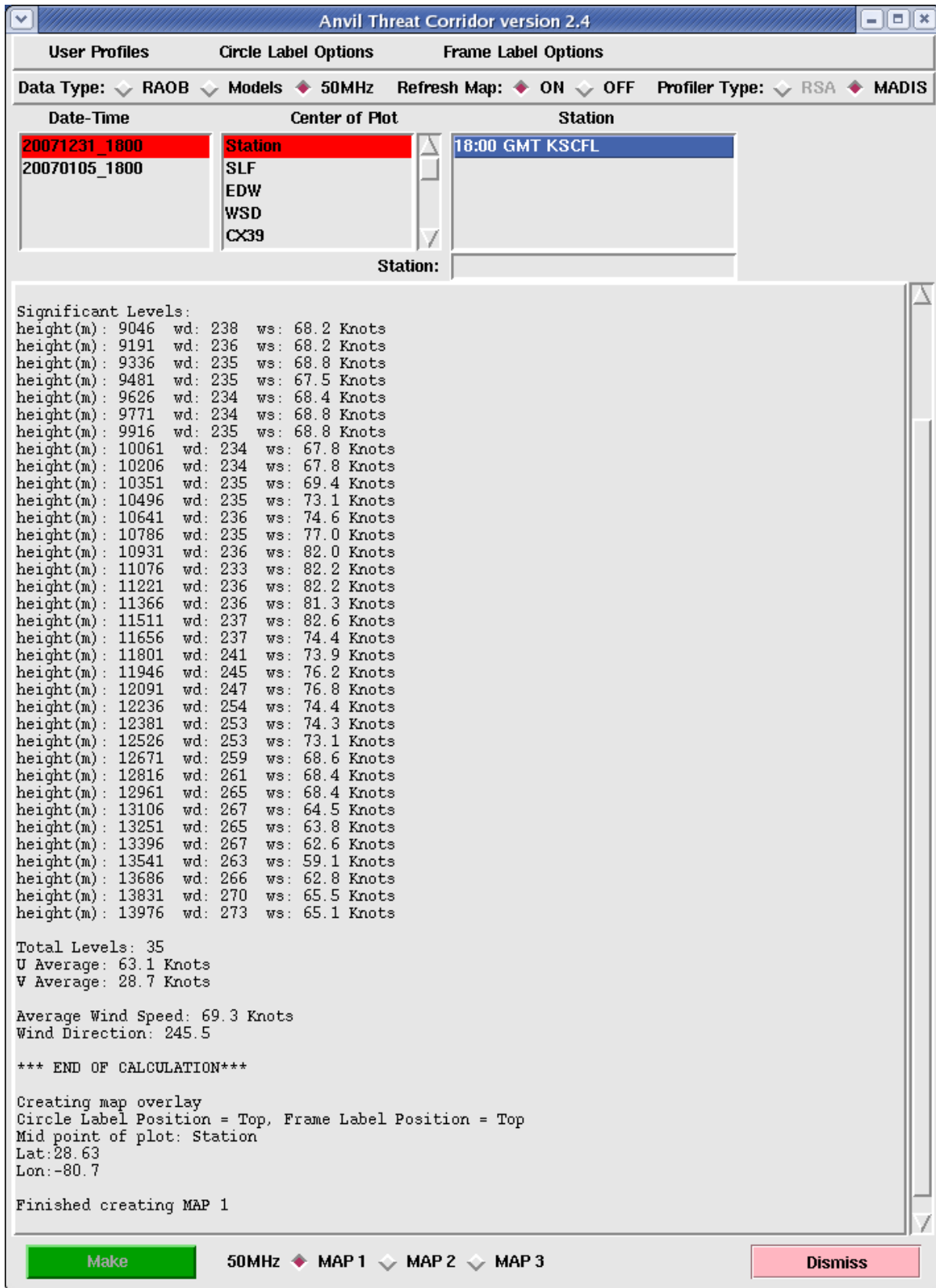
Figure 18. Anvil Tool GUI after the user has clicked on the Make button. The name and latitude/longitude of the Center of Plot, as well as the label positions, are displayed at the bottom of the GUI's text box.
