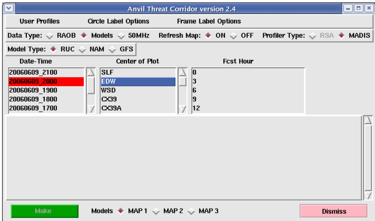
Figure 22. Anvil Tool GUI after a user has selected EDW as the Center of Plot.
