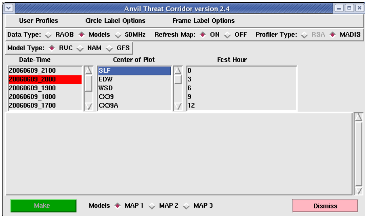
Figure 21. Anvil Tool GUI after a user has selected a Date-Time of 20060609_2000. The GUI displays the available forecast hours in the Fcst Hour listbox.
