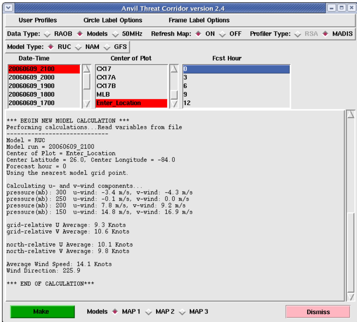
Figure 25. Anvil Tool GUI after the layer-average wind velocity was calculated for a user-defined latitude/longitude of 26.0 North/84.0 West.
